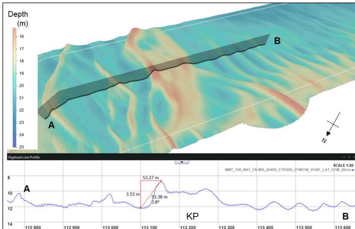
Plate 1.33 Mega ripples up to 3.53 m high located near KP 108 (MMT, 2022)
