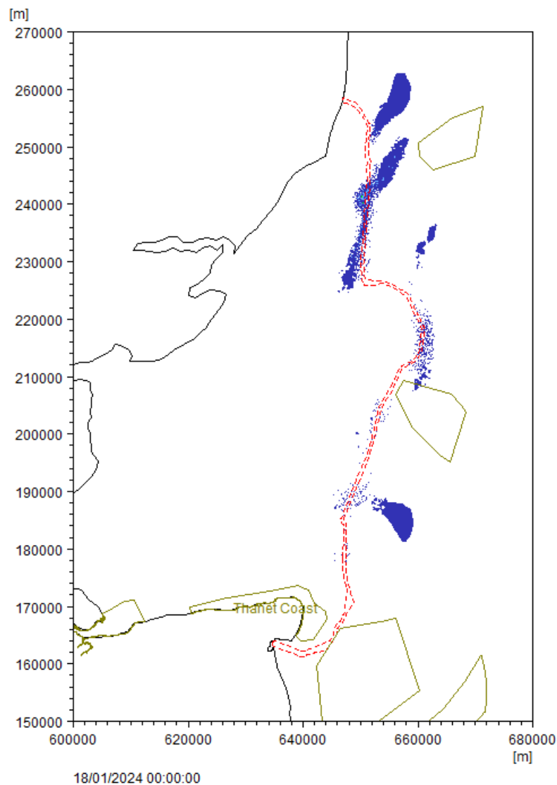
Plate 1.39 Mud SSC levels for jetting installation commencing on spring tides with output at +7 days (left) and +14 days (right) after start of activity
