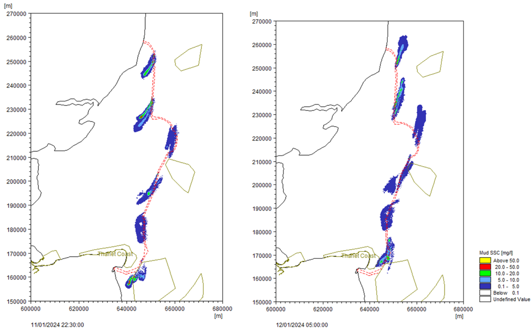
Plate 1.38 Mud SSC levels for jetting installation commencing on spring tides with output on flood (left) and ebb (right) tide after first 24 hours of activity
