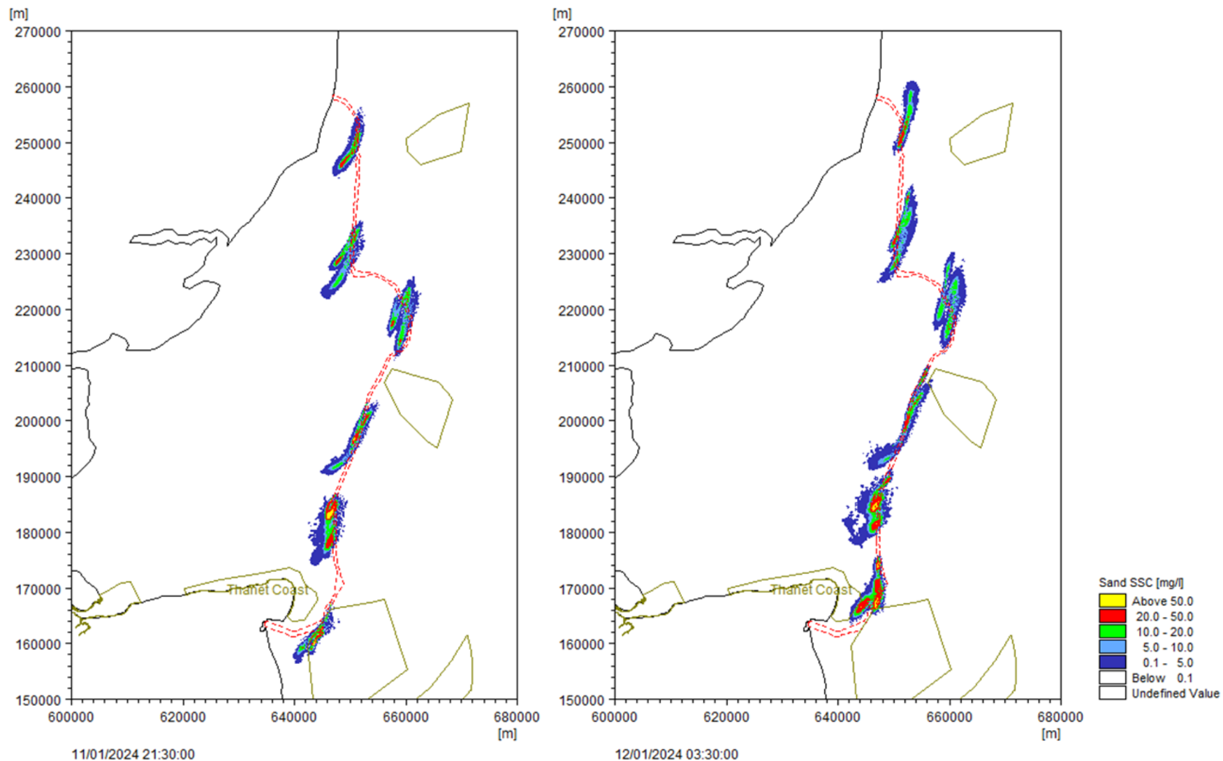
Plate 1.40 Sand SSC levels for jetting installation commencing on spring tides with output on flood (left) and ebb (right) tide after first 24 hours of activity
