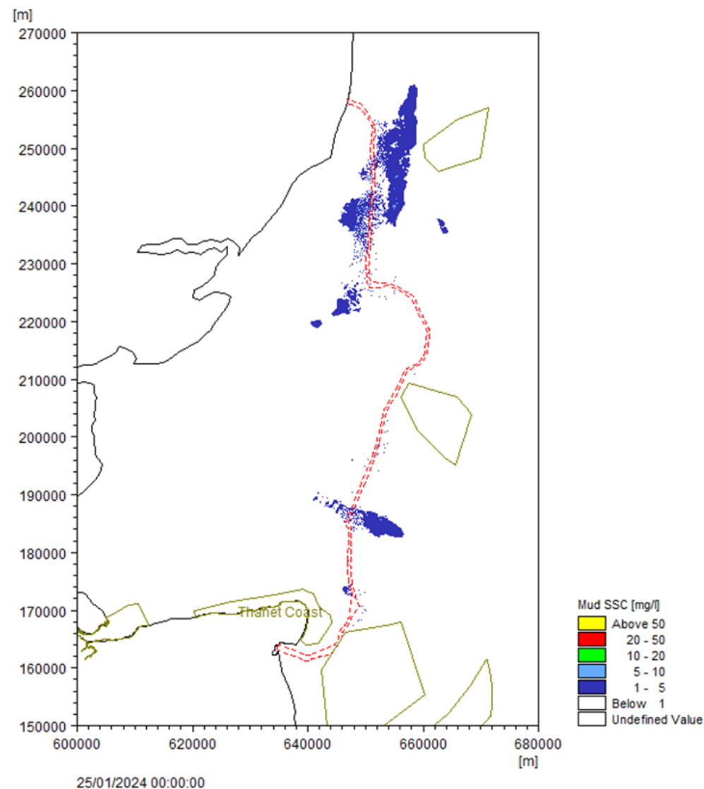
Plate 1.39 Mud SSC levels for jetting installation commencing on spring tides with output at +7 days (left) and +14 days (right) after start of activity
