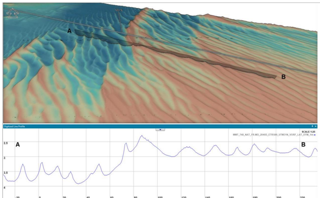
Plate 1.34 Slopes along the route associated with lee slopes of a mega-ripple area at KP 117 (MMT, 2022)
